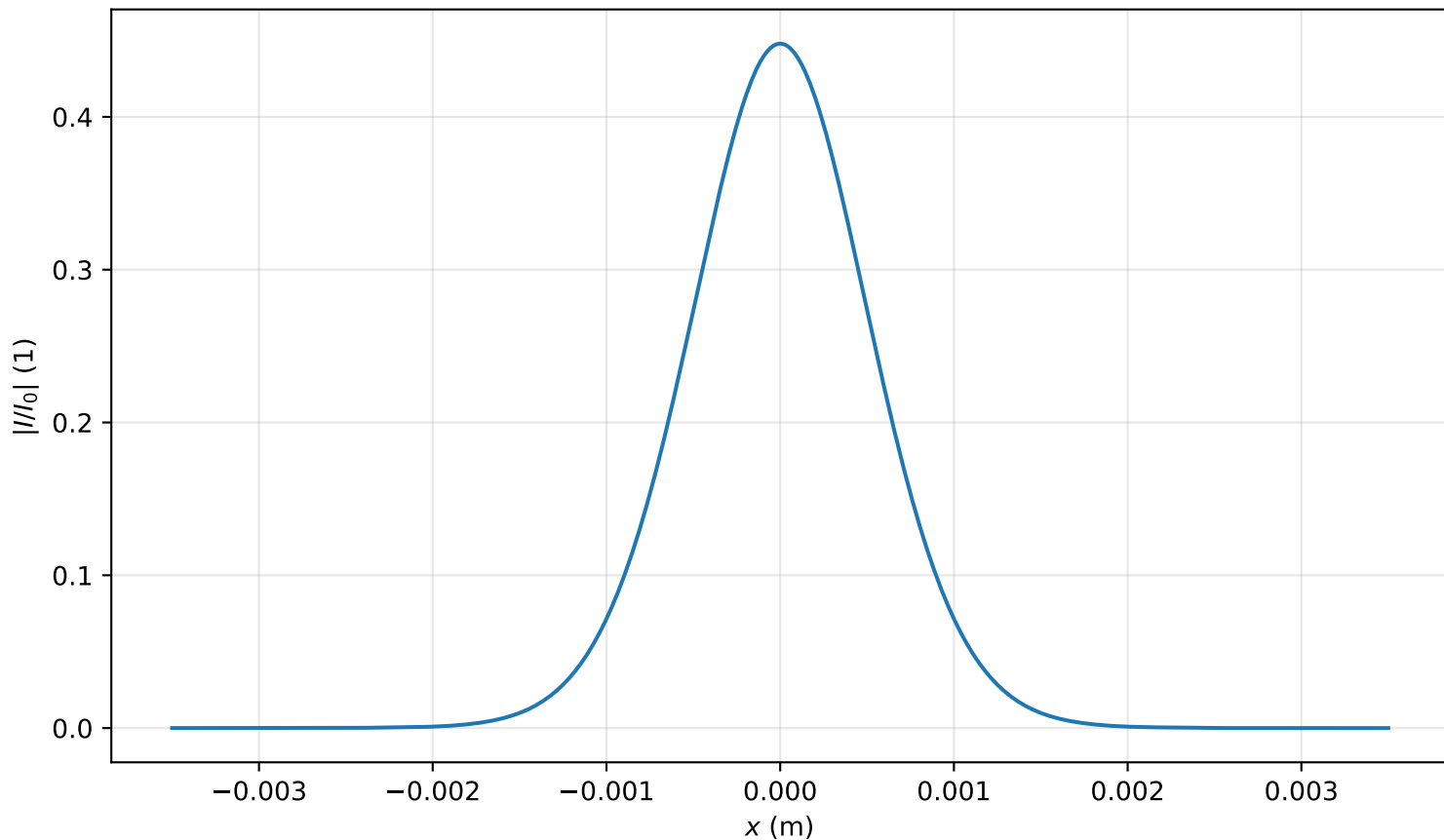
Intensity profile I(x, y = 0, z = 2.866m)/I_0 , P_{in}=0.3P_{cr} , artificial time
